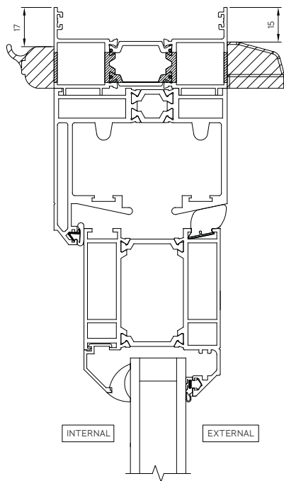
21b Bi-Fold Frame Extender With Trickle Vent
