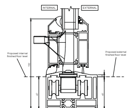
7a-7b - Non Weathered Threshold Details
