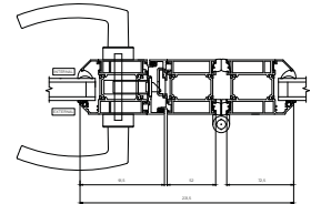
9 - Locking Mullion Detail
