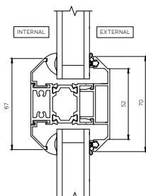
14 - Midrail Detail
