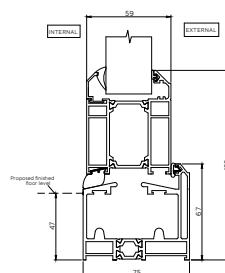
6a-6e - Bottom Track Threshold Details
