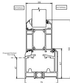
6a-6e - Bottom Track Threshold Details
